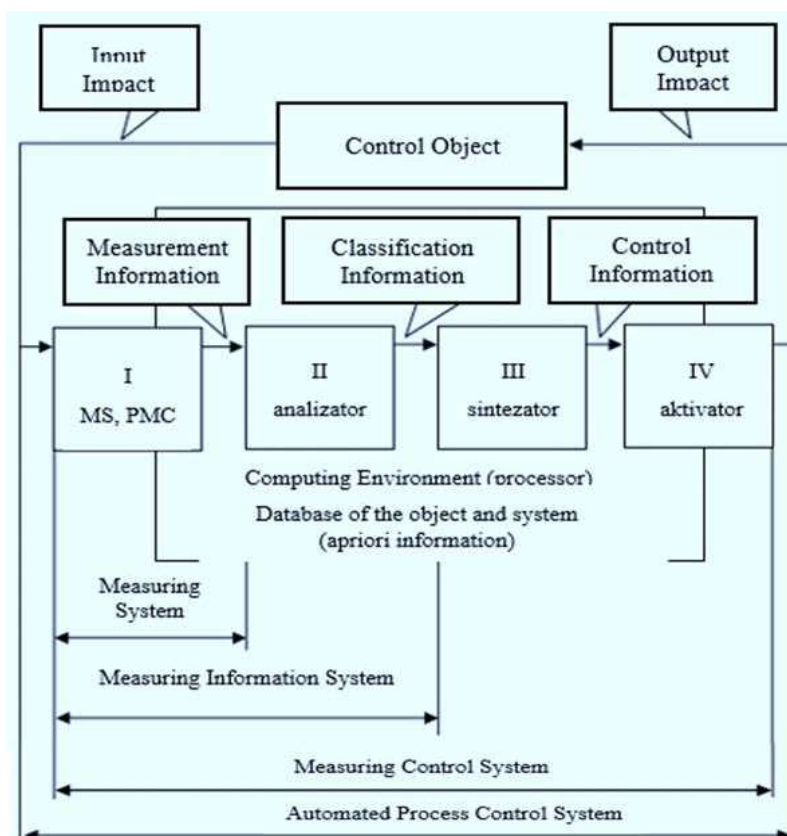
Figure 1 – Simplified structure of the IIS and APCS
